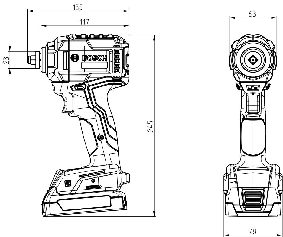
IDS 18V-125 T Dimensions in mm
