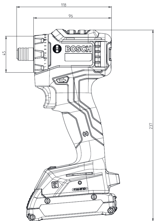
ISR 18V-30 PHX Dimensions in mm
